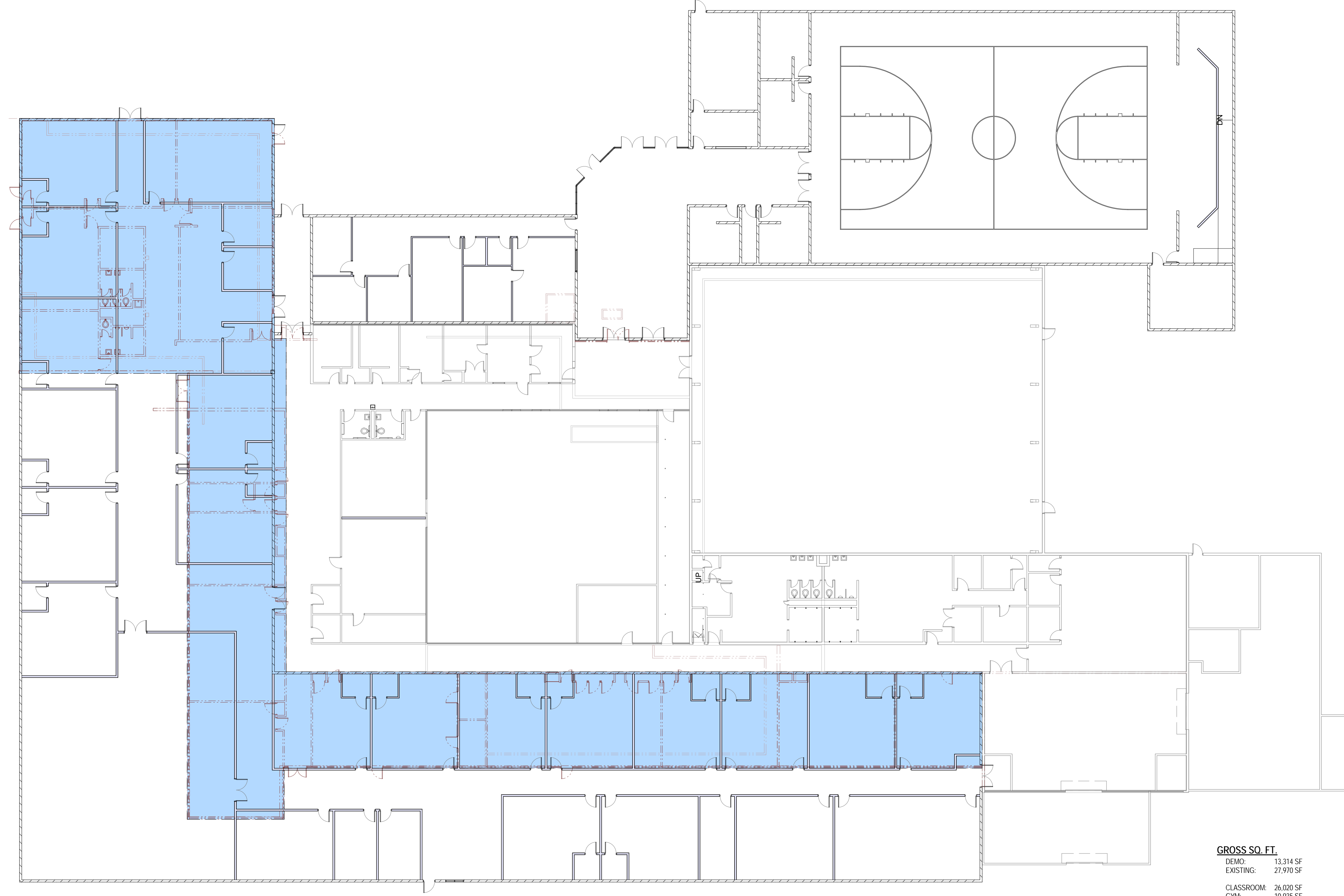
1 FIRST FLOOR - DEMOLITION & NEW SCALE: 1/16" = 1'-0"
